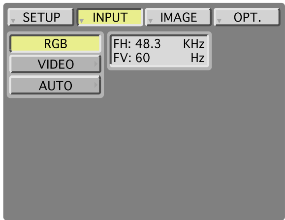
Figure 4.7 RGB Input Submenu
