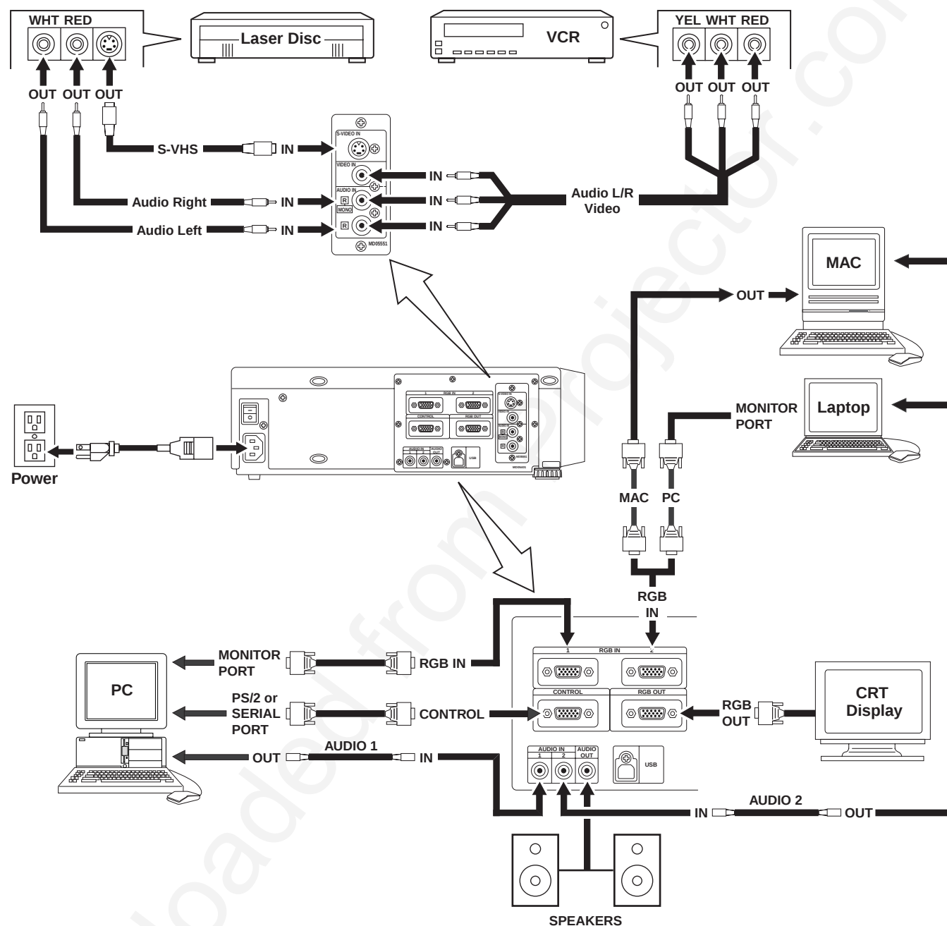
Figure 2.3 Cable Connections
