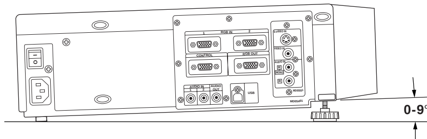
Figure 4.1 Height Adjustment
