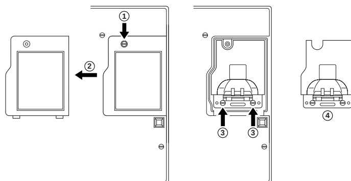
Figure 6.1 Lamp Module
