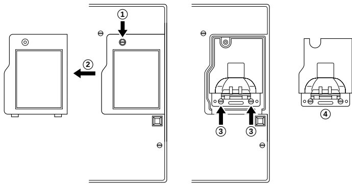
Figure 6.1 Lamp Module
