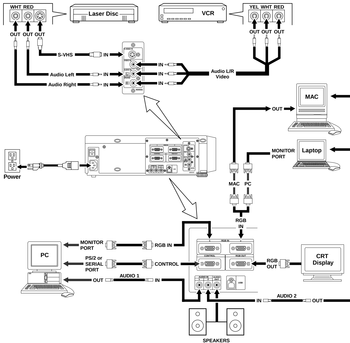
Figure 2.2 Cable Connections
