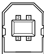
Pin Configuration
