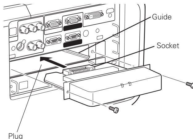
Figure shows HD DATA WIRELESS Receiver Board
