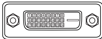
Pin Configuration
