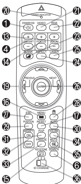
Remote Control
