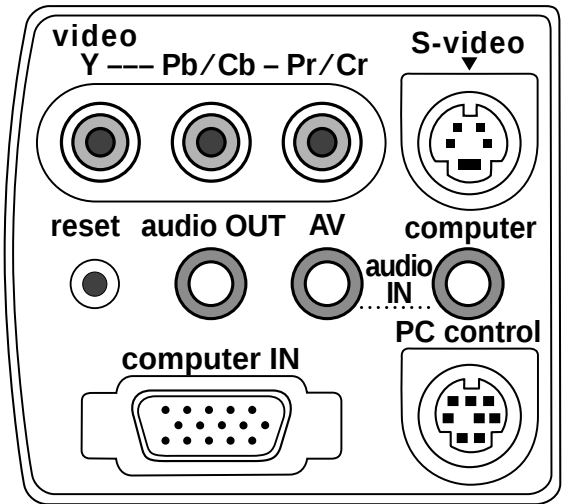
FIGURE 4 Connector panel
