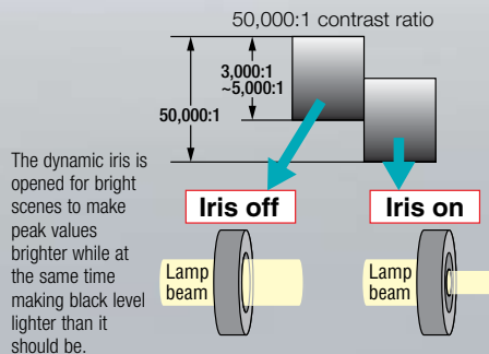
Conventional projector with dynamic iris
