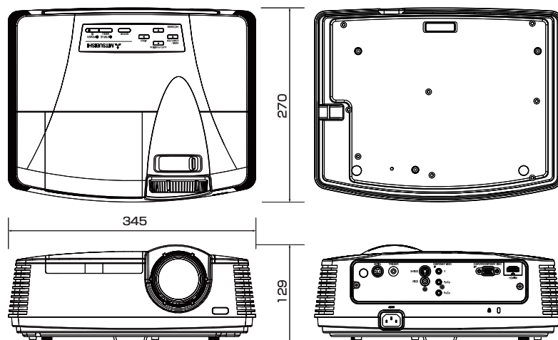
Dimension drawings (unit: mm)
