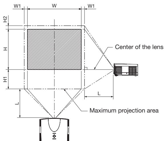
Front projection
